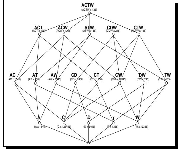
Figure 3: Frequent Itemsets
